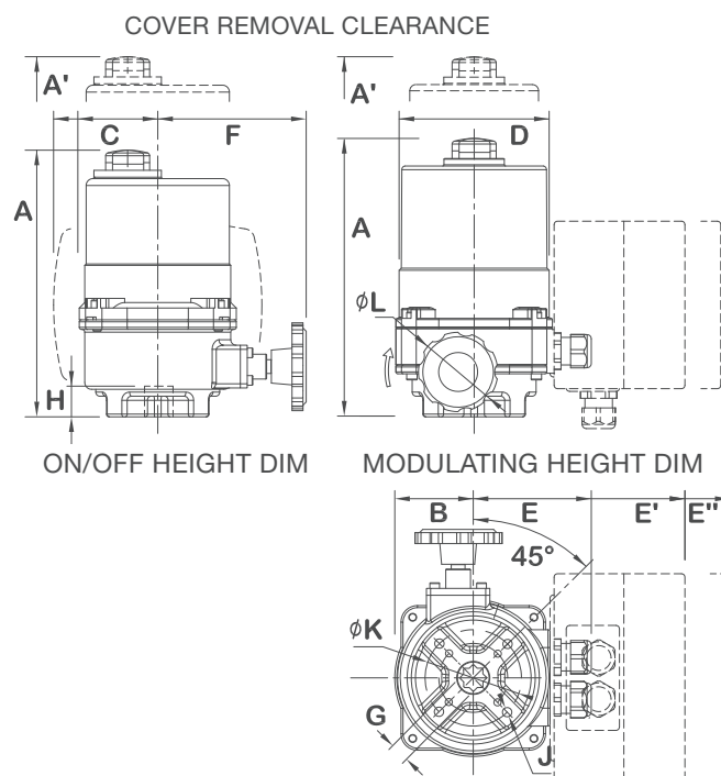
HRSN2B/2S (WITH HANDWHEEL OVERRIDE)
