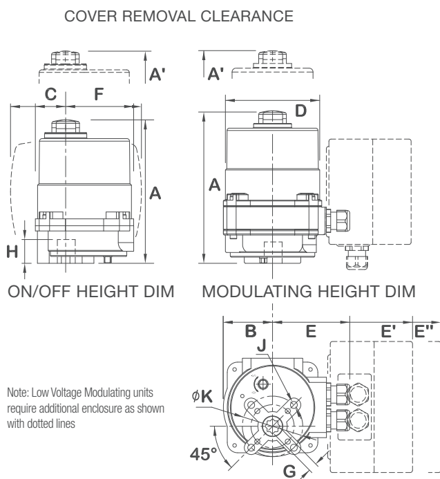
HRSN2A/2R (NO HANDWHEEL)
