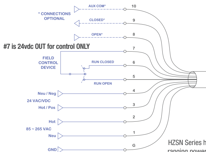
ON/OFF WIRING DIAGRAM
