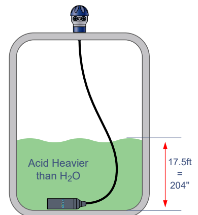
Specific Gravity = 2 Tank # 3
