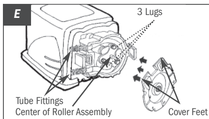
E Align cover feet near tube fittings
