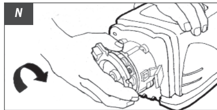
N Install cover feet first
