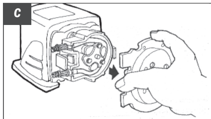
C Remove cover
