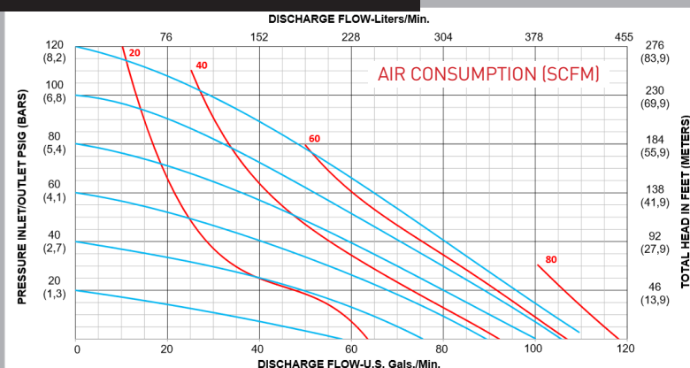
PERFORMANCE CURVE (1-1/4" RUBBER)*
