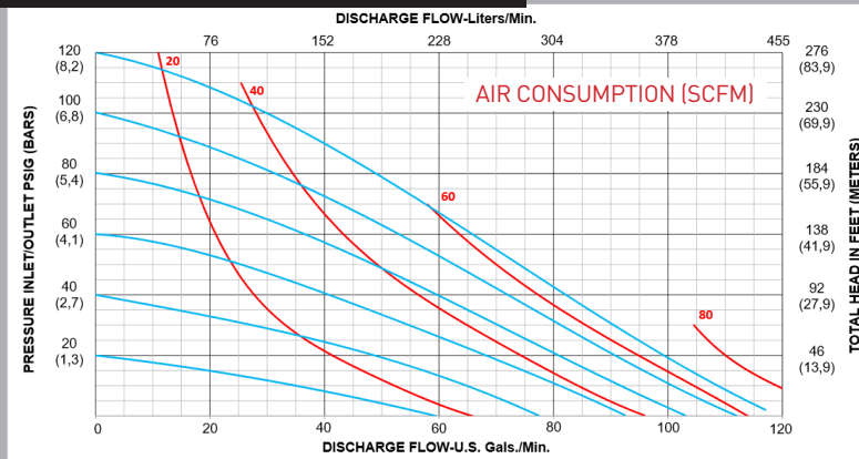
PERFORMANCE CURVE (1-1/2" RUBBER)*
